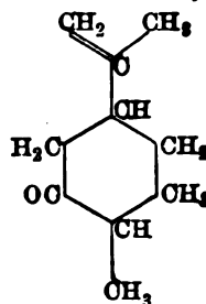
Dihydrocarvone.
